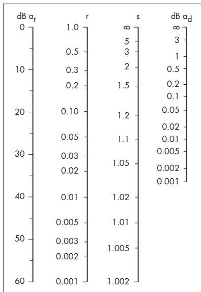
Fig. 6 Nomogram for reflection coefficient r , SWR, return loss \alpha_r , and mismatch loss \alpha_d
