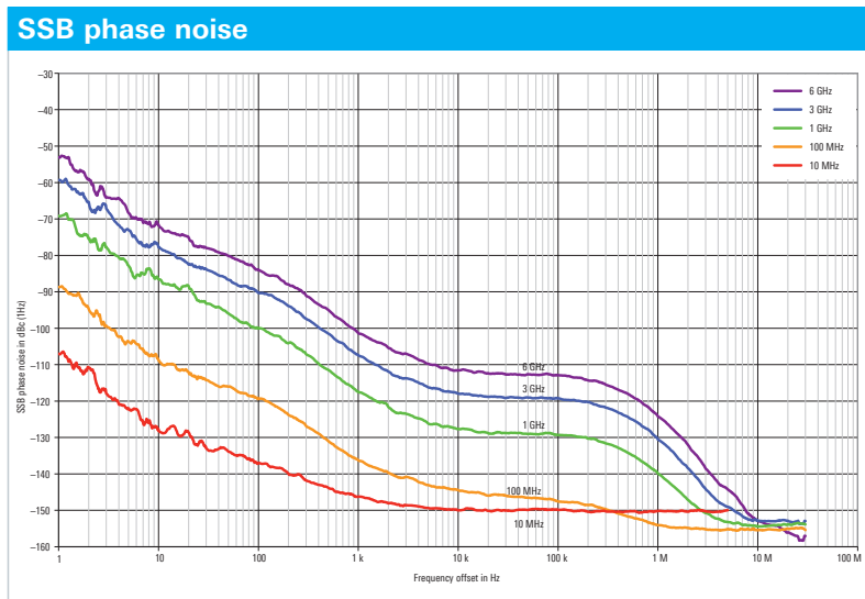
Measured SSB phase noise with the R&S®SMB-B1H OCXO option for the 1/2/3/6 GHz model.
