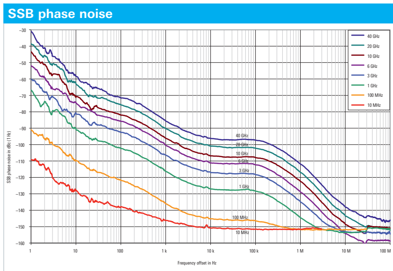
Measured SSB phase noise with the R&S®SMB-B1H OCXO option for the 12.75/20/40 GHz model.
